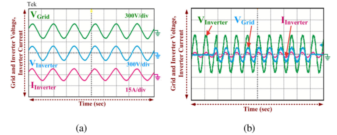
Fig. 15. Grid synchronization. (a) Inverter voltage, grid voltage, and inverter current under steady-state conditions. (b) Grid and inverter under dynamic operating conditions.
